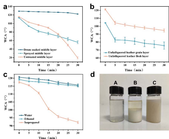
Fig. 10 (a) The influence of different treatment methods on the WCA of the middle layer. (b) WCAs of unfatigued sheepskins treated with TMS16. (c) The influence of soaking in different solvents for 24 hours on WCAs. (d) The waste liquid with different TMS16 treatment: (A) the optimal proportion, (B) excess ethanol in the system, (C) first-treated with TMS16, then fatiquoring.
