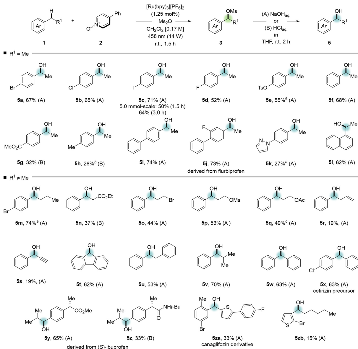
Scheme 3 Reaction scope of the benzylic C–H bond oxygenation. Reactions were run on a 0.5 mmol scale, using 1 (1.0 equiv.), 4-phenylpyridine N -oxide ( 4g ) (3.0 equiv.), \text{Ms}_2\text{O} (3.0 equiv.) and [\text{Ru}(\text{bpy})_3][\text{PF}_6]_2 (1.25 mol%) in \text{CH}_2\text{Cl}_2 [0.17 M]. Irradiation with two LED panels (458 nm, 2 x 7 W). Yields refer to isolated material over two steps and are listed as the average of two experiments within a standard deviation of 5%. a Irradiated for 2.5 h. b Irradiated for 0.5 h. c Hydrolysis for 0.5 h.
