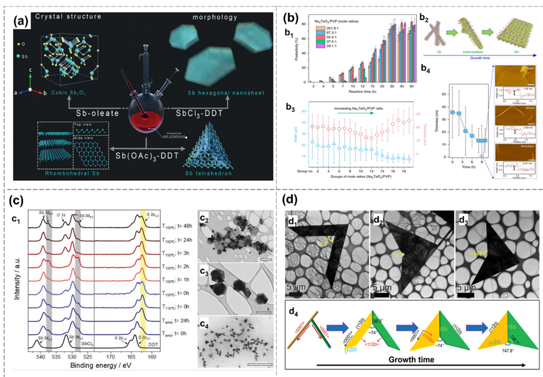
Fig. 11 Wet-chemical synthesis of antimonene and tellurene. (a) Schematic diagram of the wet-chemical synthesis of hexagonal antimonene, antimony trioxide and antimony tetrahydral. 34 (b) Solution growth and process of tellurene. 120 Productivity of tellurene over reaction time with different PVP concentrations (b 1 ). Morphology evolution from Te nanowires to 2D tellurene over growth time (b 2 ). Thickness and width of Te over mole ratios ( \text{Na}_2\text{TeO}_3/\text{PVP} ) (b 3 ). The thickness of 2D tellurene over a reaction time of thinning (b 4 ). (c) Characterization of 2D antimonene prepared by colloidal approach. 106 XPS spectra of Sb and S under different reaction conditions (c 1 ). TEM image of antimonene prepared at ambient temperature and t = 0 h (c 2 ). Sb particles obtained after t = 2 h (c 3 ) and t = 48 h (c 4 ). 106 (d) Synthesis mechanism of symmetric Te nanoflakes. 121 TEM images of the "V-shaped" Te nanoflake (d 1 ), "heart-shaped" Te nanoflake (d 2 ) and "paper airplane-shaped" Te nanoflake (d 3 ). Illustration of morphology evolution from Te nanowire to symmetrical Te nanoflake (d 4 ). Reproduced from: (a) ref. 34 with permission from Wiley-VCH, Copyright 2019; (b) ref. 120 with permission from Springer Nature, Copyright 2018; (c) ref. 106 with permission from Wiley-VCH, Copyright 2021; (d) ref. 121 with permission from Wiley-VCH, Copyright 2021.
