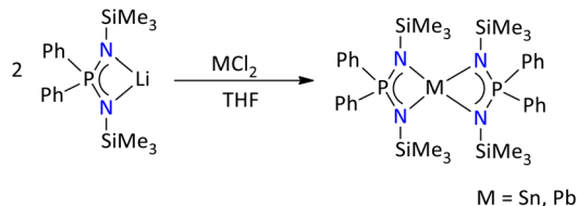
Scheme 21 Synthesis of iminophosphonamide-stabilized homoleptic stanylene and plumbylene. 67
