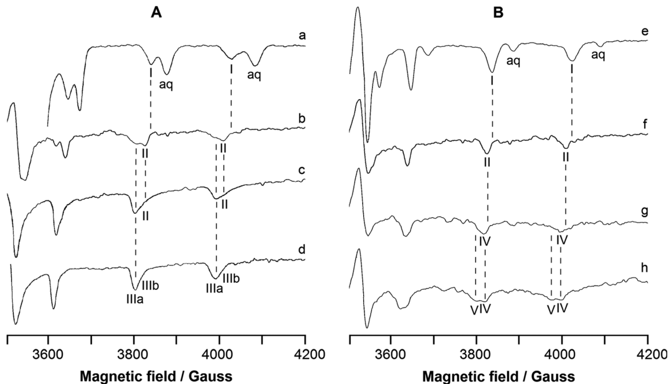
Fig. 9 In solution EPR spectra at 120 K of the systems: (A) [V^{IV}O(8-HQ)_2] -RNase A (metal : ligand : protein molar ratio = 1 : 2 : x with x = 0–1) and (B) [V^{IV}O(8-HQ)_2] -RNase A (metal : ligand : protein molar ratio = 1 : 1 : y with y = 0–1). The spectra were recorded with V^{IV}O^{2+} : 8-HQ : RNase A 1 : 2 : 0 at pH 3.0 (trace a), V^{IV}O^{2+} : 8-HQ : RNase A 1 : 2 : 1 at pH 5.1 (trace b), at pH 6.4 (trace c) and pH 7.4 (trace d); V^{IV}O^{2+} : 8-HQ : RNase A 1 : 1 : 0 at pH 4.0 (trace e); V^{IV}O^{2+} : 8-HQ : RNase A 1 : 1 : 1 at pH 5.1 (trace f), at pH 7.4 (trace g) and at pH 8.4 (trace h). V concentration is 1.0 mM in traces a and e, and 0.8 mM in traces b–d and f–h. I indicates MI = 5/2, 7/2 resonances of [V^{IV}O(8-HQ)(H_2O)_2]^+ , II of the adduct [V^{IV}O(8-HQ)(H_2O)]^+ -RNase A with Asp/Glu-COO-coordination, IIIa and IIIb of the two isomers cis - [V^{IV}O(8-HQ)_2(H_2O)] , IV of the adduct [V^{IV}O(8-HQ)(H_2O)]^+ -RNase A with His-N coordination, and V of the adduct [V^{IV}O(8-HQ)(OH)] -RNase A with His-N coordination or [V^{IV}O(8-HQ)(H_2O)]^+ -RNase A with Ser/Thr-O − coordination, while aq denotes MI = 7/2 resonances of the aqua ion [V^{IV}O(H_2O)_5]^{2+} . The positions of MI = 5/2, 7/2 resonances of I, II, IIIa, IIIb, IV, and V species are also indicated by the dotted lines. Reproduced from ref. 130, which is licensed under a Creative Commons Attribution 3.0 Unported Licence, with permission from RSC, copyright 2023.
