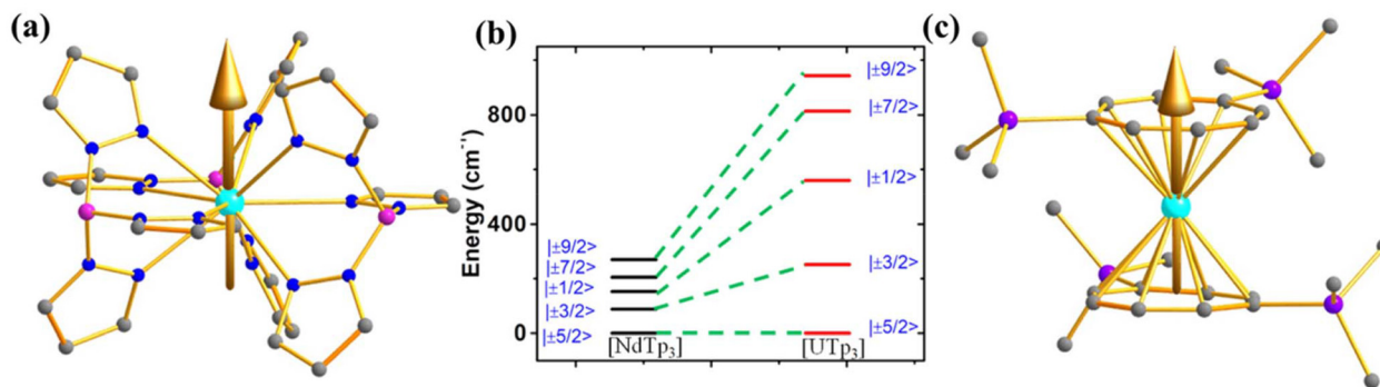
Fig. 4 (a) The magnetic anisotropy axis of [UTp_3] ( 2 ). (b) A comparison of CF splitting of five ground KDs of 1 and 2 . (c) The magnetic anisotropy axis of [Li(DME)_3][U(COT^{\prime\prime})_2] ( 3 ). Colour code: U (cyan), N (blue), Si (violet), B (pink), p (green) and C (grey). Hydrogens are omitted for clarity.
