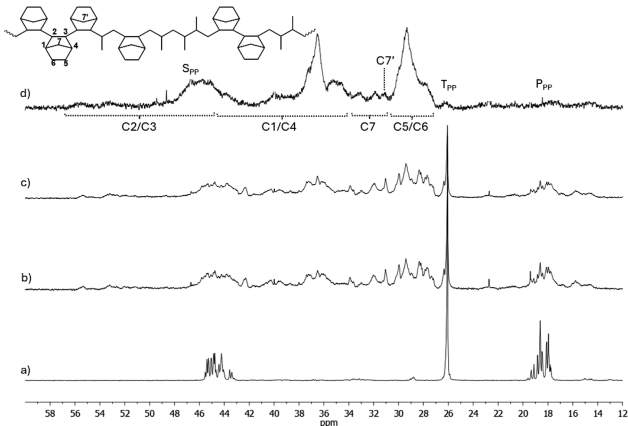
Fig. 2 ^{13}\text{C} -NMR spectra of (a) polypropylene (entry 1) and poly(P-co-N)s of (b) entry 2 ( N = 27.8 \text{ mol}\% ), (c) entry 3 ( N = 32.1 \text{ mol}\% ) and (d) entry 6 ( N = 61.7 \text{ mol}\% ) obtained using \text{CpTiCl}_2(\text{N}=\text{C}^t\text{Bu}_2) (1).
