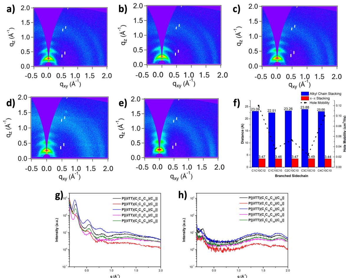
Fig. 3 Grazing incident wide-angle X-ray scattering (GIWAXS) 2D patterns of (a) P[(iITT)(C 1 C 10 C 12 )(C 12 )]]; (b) P[(iITT)(C 1 C 10 C 10 )(C 12 )]]; (c) P[(iITT)(C 2 C 10 C 10 )(C 12 )]]; (d) P[(iITT)(C 3 C 10 C 10 )(C 12 )]], and (e) P[(iITT)(C 4 C 10 C 10 )(C 12 )]]; (f) summary of chain distances (alkyl packing distance and \pi - \pi stacking) and hole mobility versus branching point; (g) out-of-plane and (h) in-plane 1D GIWAXS patterns. All measurements have been performed on thin films prepared from chlorobenzene solutions (10 mg mL -1 ) after thermal annealing at 150 °C.
