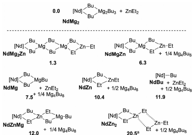
Scheme 3 Speciation of the alkylated species yielded from [\text{Nd}]\text{-}^n\text{Bu} , \text{Mg}_4^{\text{n}}\text{Bu}_8 and \text{ZnEt}_2 . Only the most stable species are shown, the fully detailed speciation is provided in ESI.† \Delta G in kcal mol -1 . a In NdZn 2 , interaction between the \text{ZnEt}_2 fragments is weak, the endergonicity results from the entropy cost of the association of free and separated \text{ZnEt}_2 . Gaussian 09, B3PW91/D3BJ(SP), SMD(TolH), 298 K, 1 atm.
