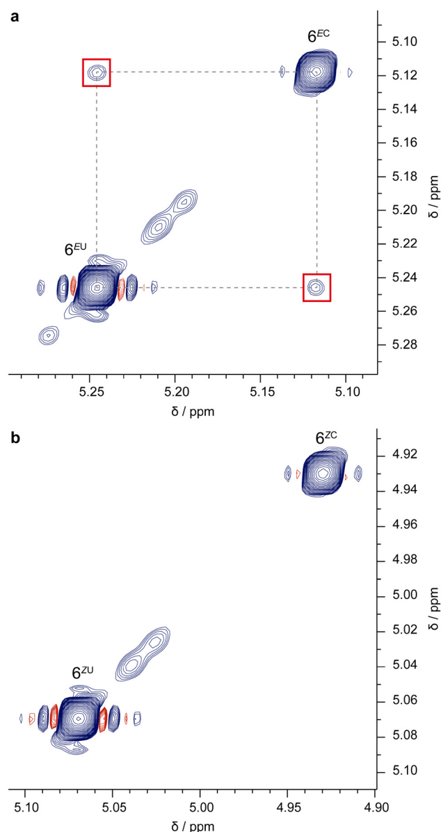
Fig. 5 Partial EXSY NMR ( CD_3CN , 500 MHz, 298 K, 1.4 mM, t_{\text{mix}} = 600 \text{ ms} ) spectra of (a) an equimolar mixture of EE\text{-}4H^+ and 2 , and (b) the same sample after exhaustive irradiation at 365 nm. 6^{EU} and 6^{EC} in (a) indicates the free and complexed EE axle, respectively, whereas 6^{ZU} and 6^{ZC} in (b) denote the free and complexed ZZ axle, respectively.
