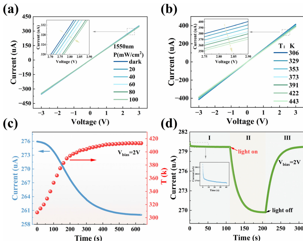
Fig. 5 Negative photoresponse characteristics of \text{Bi}_2\text{Se}_3 - \text{PtSe}_2 heterojunction photodetectors and the whole process of their photocurrent generation. I–V characteristic curves for different optical power densities (a) and different temperatures under 1550 nm illumination (b). The current generated by the device gradually decreased when the light intensity increased, and the resistance increased accordingly. At the same time, with the increase in temperature, the trend for the device current was the same as that for the increase in light intensity. (c) Curves of the current of the device as a function of temperature in the absence of light. The curves show that the temperature change caused a change in the current of the device and the current tended to decrease as the temperature increased. (d) The entire process of photocurrent generation, V_{\text{bias}} = 2\text{V} .
