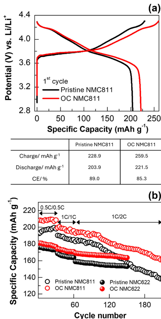
Fig. 3 Electrochemical performance of two NMC811 materials: (a) initial charge–discharge profile (0.1 C/0.1 C) at room temperature and (b) cycle retention at 60 °C.
