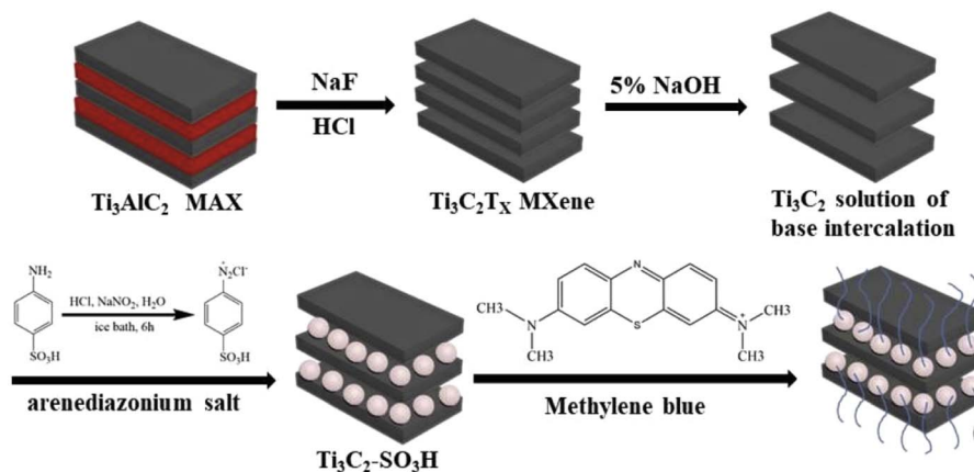
Fig. 15 Ti_3C_2T_x-SO_3H composite for the removal of methylene blue in an alkaline environment. Reproduced from ref. 120 with permission from Elsevier, copyright 2019.
