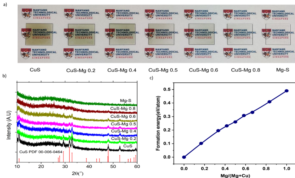
Fig. 2 (a) Photograph of Mg-modified CuS films with varying amounts of Mg, ranging from pure CuS (leftmost) to pure Mg-S (rightmost). (b) X-ray diffraction spectra of CuS-Mg films with varying Mg concentrations, from pure CuS (black) to pure Mg-S (dark green). (c) Formation energy of \text{Cu}_{1-x}\text{Mg}_x\text{S} ( 0 < x < 1 ) starting from pure CuS in covellite.
