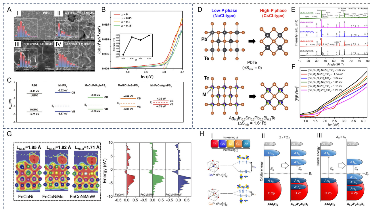
Fig. 4 Electronic structure-regulating strategies of high-entropy materials. Dimension control: (A) scanning electron microscopy images of the thermally etched surfaces of (1 - x)(Pb 0.25 Ba 0.25 Ca 0.25 Sr 0.25 )TiO 3 -xBi(Mg 2/3 Nb 1/3 )O 3 ceramics. I: (Pb 0.25 Ba 0.25 Ca 0.25 Sr 0.25 )TiO 3 ; II: 0.95(Pb 0.25 Ba 0.25 Ca 0.25 Sr 0.25 )TiO 3 -0.05Bi(Mg 2/3 Nb 1/3 )O 3 ; III: 0.9(Pb 0.25 Ba 0.25 Ca 0.25 Sr 0.25 )TiO 3 -0.1Bi(Mg 2/3 Nb 1/3 )O 3 ; IV: 0.85(Pb 0.25 Ba 0.25 Ca 0.25 Sr 0.25 )TiO 3 -0.15Bi(Mg 2/3 Nb 1/3 )O 3 , and (B) Ultraviolet-visible absorption spectrum of (1 - x)(Pb 0.25 Ba 0.25 Ca 0.25 Sr 0.25 )TiO 3 -xBi(Mg 2/3 Nb 1/3 )O 3 . The inset shows the direct band gap calculated by the Tauc plot method. Reproduced with permission from ref. 100. Copyright (2023) Elsevier. (C) Band structure diagram of MnFeCuAgInPS 3 , MnNiCuInSnPS 3 , MnCuPdAgInPS 3 , and MnPS 3 nanosheets (R6G is the probe molecule). Reproduced with permission from ref. 104. Copyright (2023) John Wiley and Sons. Phase modification: (D) schematic images of the crystal structures of low-pressure (NaCl-type) and high-pressure (CsCl-type) crystal structures of PbTe and Ag 0.2 In 0.2 Sn 0.2 Pb 0.2 Bi 0.2 Te. Reproduced with permission from ref. 106. Copyright (2023) Elsevier. (E) X-ray diffraction patterns at varying Ti content with (Co, Cu, Mg, Ni, Zn)O being the phase-pure rocksalt structure without Ti and 33.33% Ti being the stoichiometric content in the orthotitanate (Co, Cu, Mg, Ni, Zn) 2 TiO 4 , and (F) Kubelka-Munk plots and band gaps of (Co, Cu, Mg, Ni, Zn) 2 TiO 4 . Reproduced with permission from ref. 107. Copyright (2021) Elsevier. Composition modification: (G) electron localization function calculations and density of states in FeCoNi, FeCoNiMo, and FeCoNiMoW. Reproduced with permission from ref. 108. Copyright (2023) John Wiley and Sons. (H) Trends in crystal field splitting ( \Delta ), and electronegativity ( \chi ) for the five constituent metals of a high-entropy spinel. I: Crystal field splitting for tetrahedrally coordinated divalent Co and Cu. II: The addition of a transition metal of greater electronegativity can reduce the band gap energy. III The addition of a transition metal of lower crystal field splitting can reduce the band gap. Reproduced with permission from ref. 109. Copyright (2023) American Chemical Society.
