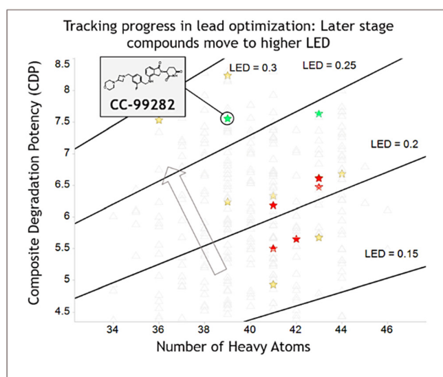
Fig. 4 LED and LipED plots of compounds in LO of CC-99282 series. Arrow indicates the desired space on the plots. Lead compounds at different stages are highlighted with colored star shape.
