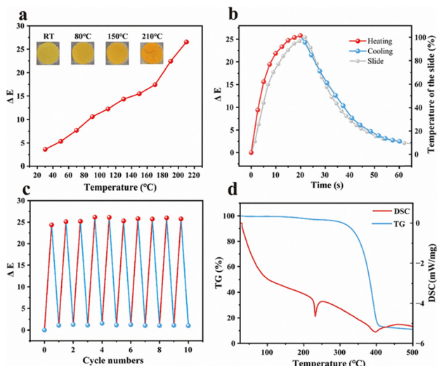
Fig. 9 H 2 L 21 showing thermochromic responsiveness (a) ΔE–T plot, (b) response time curve and temperature of the slide, (c) heating–cooling cycles, and (d) TG–DSC curve; reproduced from ref. 80 with permission from Elsevier, Copyright 2024.
