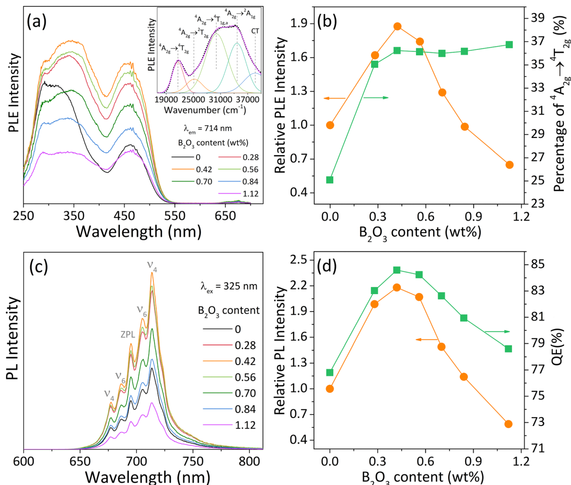
Fig. 2 (a) Room-temperature PLE spectra of \text{Ca}_{14}\text{Zn}_6\text{Al}_{9.8}\text{Mn}_{0.1}\text{Mg}_{0.1}\text{O}_{35} - z \text{ wt\% B}_2\text{O}_3 phosphors. The inset shows the deconvoluted PLE spectrum of \text{Ca}_{14}\text{Zn}_6\text{Al}_{9.8}\text{Mn}_{0.1}\text{Mg}_{0.1}\text{O}_{35} without \text{B}_2\text{O}_3 additive using Gaussian fitting. (b) Dependence of the PLE intensity and the percentage of ^4\text{A}_{2g} \rightarrow ^4\text{T}_{2g} transition (i.e., blue light absorption) in the \sim 250\text{--}550 \text{ nm} spectral region on the weight content of \text{B}_2\text{O}_3 . (c) Room-temperature PL spectra of \text{Ca}_{14}\text{Zn}_6\text{Al}_{9.8}\text{Mn}_{0.1}\text{Mg}_{0.1}\text{O}_{35} - z \text{ wt\% B}_2\text{O}_3 phosphors. (d) Dependence of the PL intensity and QE on the weight content of \text{B}_2\text{O}_3 .
