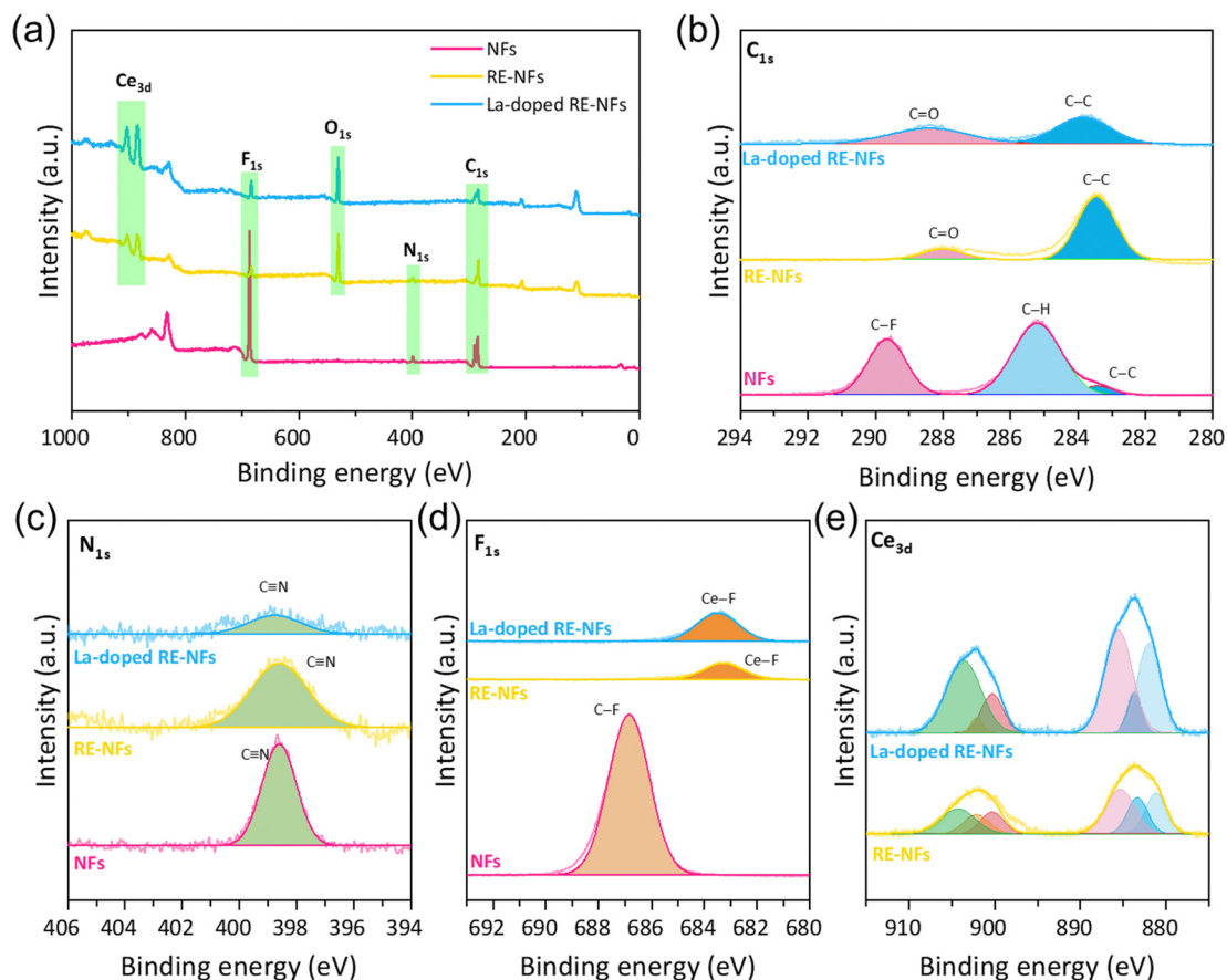
Fig. 4 XPS spectra of NFs, RE-NFs, and La-doped RE-NFs. (a) Survey spectrum displaying the elemental composition with highlighted peaks for Ce 3d, F 1s, O 1s, C 1s, and N 1s, confirming successful integration of rare-earth elements. The high-resolution spectra for (b) C 1s, (c) N 1s, (d) F 1s, and (e) Ce 3d provide detailed insights into the chemical states of each element in the prepared samples.
