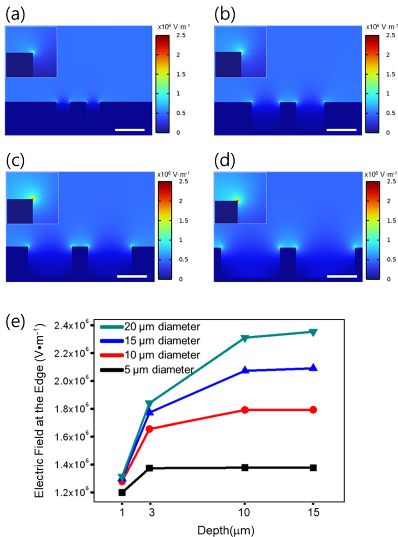
Fig. 2 Results of the numerical analysis of the effect of the diameter on the formation of nonuniform electric fields: diameter = (a) 5 \mu m, (b) 10 \mu m, (c) 15 \mu m, and (d) 20 \mu m, respectively. The scale bars are equal to 10 \mu m. (e) the diameter and depth influence the formation of non-uniform electric field. Detailed results of the numerical analysis of the effect of depth are provided in the ESI† as Fig. S1–S3.
