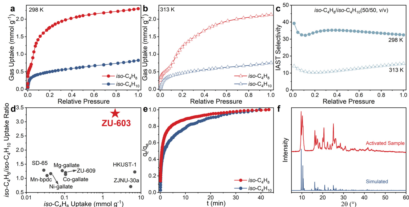
Fig. 2 Pure component adsorption isotherms of \text{iso-C}_4\text{H}_8 and \text{iso-C}_4\text{H}_{10} on ZU-603 at (a) 298 K and (b) 313 K; (c) \text{iso-C}_4\text{H}_8/\text{iso-C}_4\text{H}_{10} (50/50) IAST selectivity of ZU-603 calculated in the pressure range of 0–1 bar at 298 K and 313 K; (d) comparison of uptake ratio of \text{iso-C}_4\text{H}_8 (0.5 bar)/ \text{iso-C}_4\text{H}_{10} (0.5 bar) and \text{iso-C}_4\text{H}_8 (0.5 bar) uptake of ZU-603 against other reported materials; (e) time dependent adsorption profiles of \text{iso-C}_4\text{H}_8 and \text{iso-C}_4\text{H}_{10} at 298 K and 0.6 bar; (f) powder X-ray diffraction patterns (PXRD) of the activated sample and pattern simulated using the crystal structure of ZU-603.
