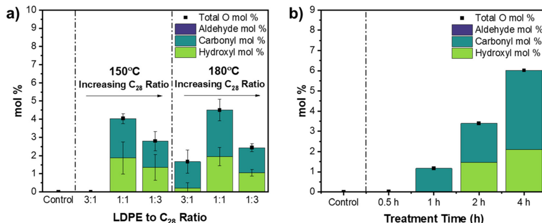
Fig. 5 Oxygen percentage and functional group incorporation in plasma-treated LDPE ( 40 \text{ kg mol}^{-1} ) at various (a) LDPE to C 28 ratios at two temperatures and (b) treatment times at 150^\circ\text{C} and LDPE to C 28 ratio of 1:1. The control (neat LDPE) is also shown. Carbonyl groups refer to middle chain C=O bonds while aldehyde groups refer to end chain C=O groups. Plasma operating conditions: treatment time: 2 h, O 2 feed molar percent: 2%, stir rate: 0 rpm.
