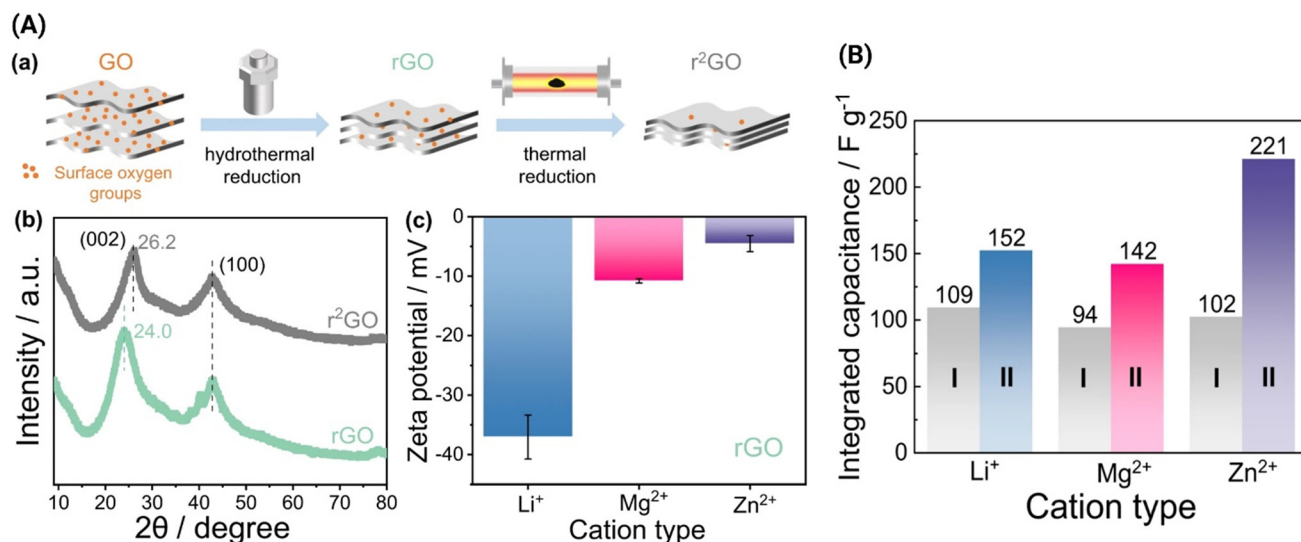
Fig. 7 Threats for MOFs (A) synthesis and characterisation of 2D reduced graphene oxide (rGO) through a two-step reduction process involving hydrothermal and thermal reduction methods. 151 (B) Electrochemical performance of prepared rGO sheets in different aqueous electrolytes, illustrated through integrated capacitance and cyclic voltammetry, showing the impact of various cations (Li + , Mg 2+ , Zn 2+ ) on capacitance. The enhancement is highest for zinc ions, followed by magnesium ions, and lowest for lithium ions, aligning with the expected interaction strength between the cations and rGO. 151
