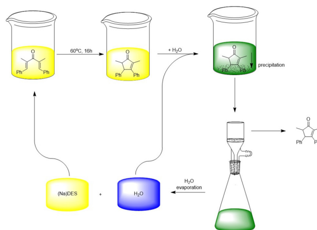
Fig. 6 Recycling process for (Na)DES and water involved in the thermal cyclisation of divinyl ketone. This figure has been adapted from ref. 61 with permission from Royal Society of Chemistry, copyright 2020.
