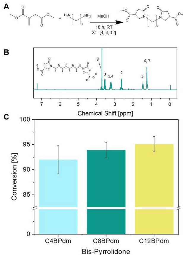
Fig. 2 Synthesis of the bis-pyrrolidone (CxBPdm) building blocks. (A) The reaction between DMI and diamine spacers with x = [4, 8, \text{and } 12] using a catalytic amount of methanol used to prepare the BPdm structures. (B) 1 H-NMR spectrum of C8BPdm; (C) the raw yield of BPdm structures (calculated using eqn (1)).
