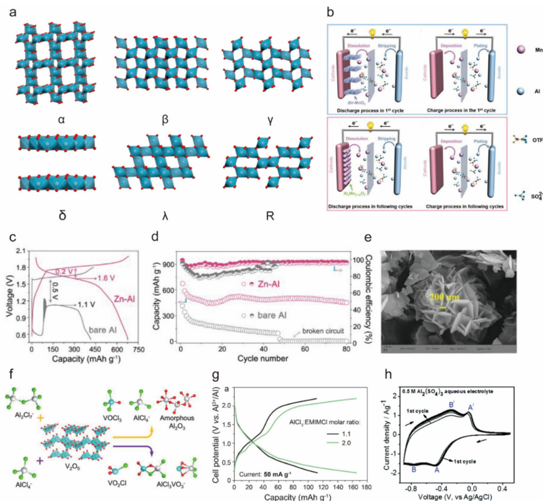
Fig. 3 (a) Schematic of the crystal structure of different types of \text{MnO}_2 . (b) The schematic electrochemistry diagram of the \text{Al}||\text{MnO}_2 batteries during the first discharge and charge processes. Copyright 2019, Wiley-VCH. (c) First galvanostatic discharge and charge (GCD) curves, and (d) cycling performance at a current rate of 100 \text{ mA g}^{-1} of the \text{Al}||\text{Al}_x\text{MnO}_2 and \text{Zn-Al}||\text{Al}_x\text{MnO}_2 batteries in the 2 \text{ M Al(OTf)}_3 electrolyte. 31 Copyright 2020, American Chemical Society. (e) Scanning electron microscope (SEM) image of the synthesized \text{V}_2\text{O}_5 nanosheets. 58 Copyright 2023, American Chemical Society. (f) Schematic illustration of the product of the reaction of \text{V}_2\text{O}_5 with the [\text{AlCl}_4]^- and [\text{Al}_2\text{Cl}_7]^- charge carriers. 41 Copyright 2019, American Chemical Society. (g) GCD curves of the \text{TiO}_2 NRs at the 3 rd cycle at a current rate of 50 \text{ mA g}^{-1} in mild ( 1.1:1 molar ratio) and acidic ( 2.0:1 molar ratio) \text{AlCl}_3/\text{EMImCl} ionic liquid electrolytes. 68 Copyright 2019, American Chemical Society. (h) CV curves of \text{WO}_3 in the 0.5 \text{ M Al}_2(\text{SO}_4)_3 aqueous electrolyte. 69 Copyright 2019, The Royal Society of Chemistry.
