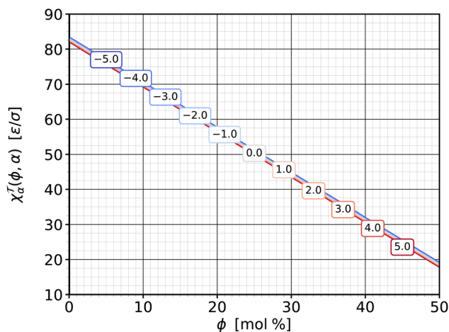
Fig. 9 Susceptibility \chi'_{\alpha|\phi} from eqn (13b) as a function of cholesterol content \phi , parameterized by different values of phospholipid abundance \alpha , as indicated in the boxed labels. The lines almost coincide, with smaller \alpha values having ever so slightly larger susceptibilities.
