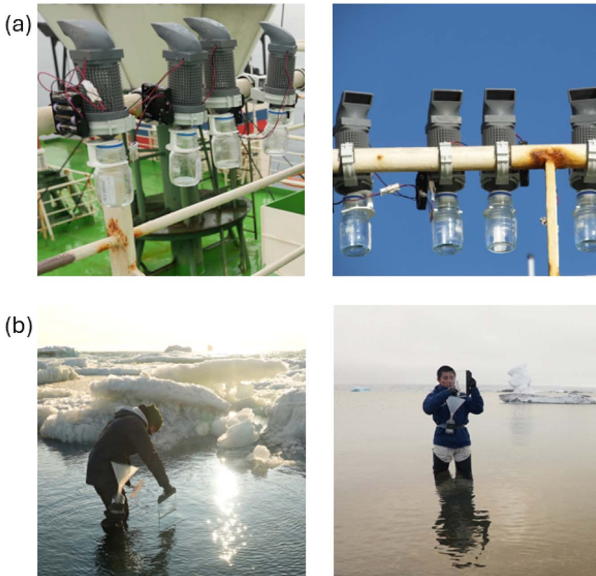
Fig. 3 (a) Fog water sample collector; (b) collection of SML.
