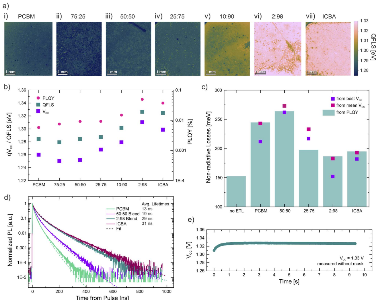
Fig. 3 Photoluminescence (PL) characterization of perovskite solar cells and half-stacks with PCBM : ICBA ETL interlayers to determine impact on non-radiative losses within the device. (a) Spatial maps of quasi-Fermi level splitting (QFLS) of complete solar cells with PCBM : ICBA interlayers (ITO/Me-4PACz/np-Al 2 O 3 /perovskite/PCBM : ICBA/C 60 /BCP/Ag). (b) Comparison of photoluminescence quantum yield (PLQY) & QFLS (average values from images), and V_{OC} (same imaged device measured under simulated AM1.5 100 mW cm -2 irradiance) of complete solar cells with PCBM : ICBA interlayers. (c) Non-radiative losses of solar cell half-stacks with PCBM : ICBA interlayers (ITO/Me-4PACz/np-Al 2 O 3 /perovskite/PCBM : ICBA/C 60 ) calculated from measured V_{OC} and average PLQY from images. (d) Time-resolved photoluminescence with stretched exponential fitting of half-stacks with PCBM : ICBA interlayers (ITO/Me-4PACz/perovskite/PCBM : ICBA). (e) Steady state V_{OC} of complete solar cell with 2 : 98 PCBM : ICBA interlayer.
