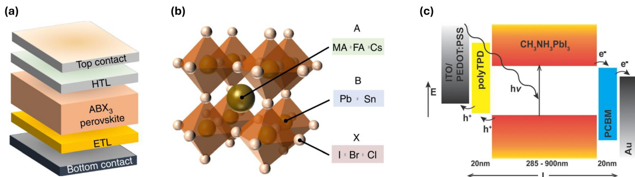
Fig. 1 (a) Typical perovskite solar cell structure. (b) \text{ABX}_3 crystal structure of perovskite absorbers. MA, FA and Cs stand for methylammonium, formamidinium, and cesium, respectively. (c) Energy level diagram of a PSC consisting of ITO as TCO, PolyTPD as the HTL, \text{CH}_3\text{NH}_3\text{PbI}_3 as the absorber, PCBM as the ETL and gold (Au) as the top contact metal electrode. (a) and (b) are adapted with permission from ref. 5, copyright ©2022, Springer Nature. (c) is adapted with permission from ref. 6, copyright 2017, John Wiley and Sons.
