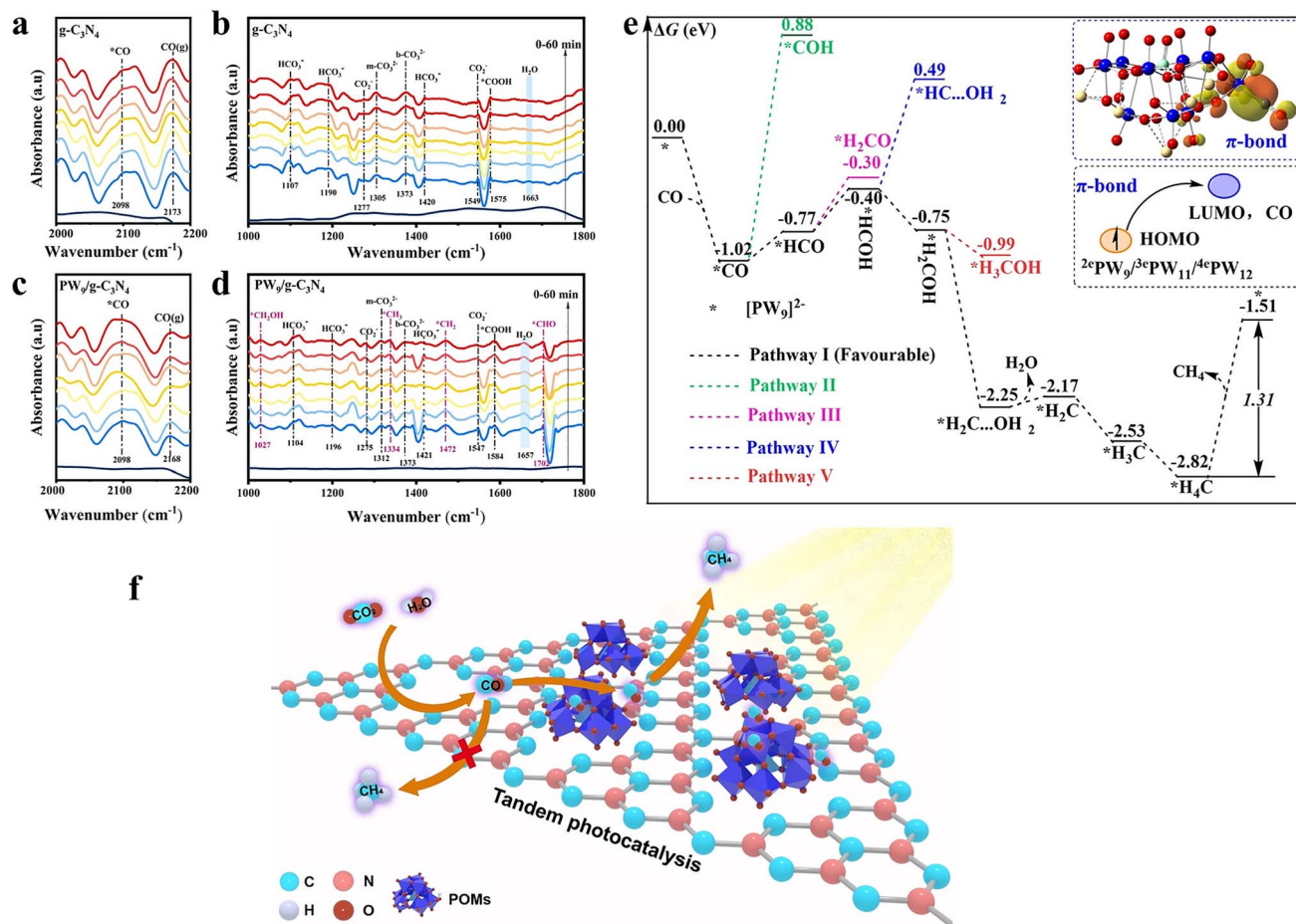
Fig. 9 In situ DRIFTS spectra during the photocatalytic \text{CO}_2 reduction process of (a) \text{g-C}_3\text{N}_4 in 2000\text{--}2200\text{ cm}^{-1} ; (b) \text{g-C}_3\text{N}_4 in 1000\text{--}1800\text{ cm}^{-1} ; (c) \text{PW}_9/\text{g-C}_3\text{N}_4 in the range of 2000\text{--}2200\text{ cm}^{-1} and (d) \text{PW}_9/\text{g-C}_3\text{N}_4 in the range of 1000\text{--}1800\text{ cm}^{-1} ; (e) free energy change of \text{CH}_4 formation and release mediated by [\text{PW}_9]^{2-} and the \pi -bond between W of [\text{PW}_9]^{2-} and C of CO; and (f) the reaction mechanism from \text{CO}_2 to \text{CH}_4 . 119
