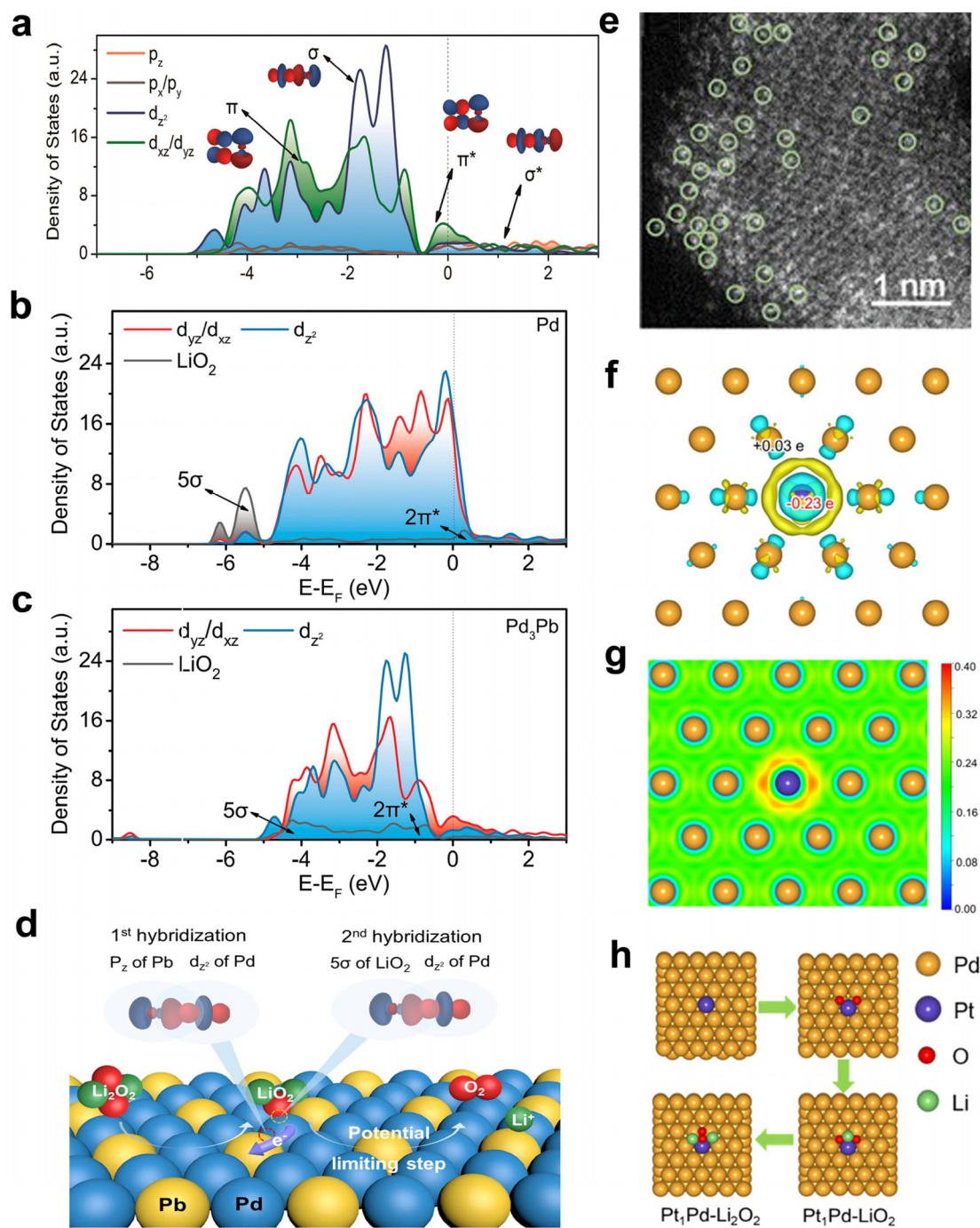
Fig. 13 (a) DOS of Pd d_{z^2} , d_{xz}/d_{yz} orbitals and Pb p_x , p_y , p_z orbitals after intra-molecular p-d orbital hybridization in Pd 3 Pb. (b) DOS of Pd 4d d_{yz}/d_{xz} and d_{z^2} orbitals in Pd. (c) DOS of Pd 4d d_{yz}/d_{xz} and d_{z^2} orbitals in Pd 3 Pb with adsorbed LiO 2 . (d) Schematic representation of cascade orbital-oriented hybridization from intra-molecular Pb-Pd p-d hybridization in Pd 3 Pb to inter-molecular orbital hybridization between Pd 3 Pb (Pd d_{xz}/d_{yz} and d_{z^2} ) and LiO 2 ( 2\pi^* and 5\sigma ), using the d_{z^2} orbital along the z-axis as an example. 115 (e) AC-HAADF-STEM image of the Pt 1 Pd alloy (single-atom Pt marked with green circles). (f) ELF values of Pt 1 Pd. (g) Charge density difference distribution (regions of electron enrichment and depletion) in Pt 1 Pd. (h) Schematic representation of the discharge pathway of a Li-O 2 battery on the Pt 1 Pd surface. 40
