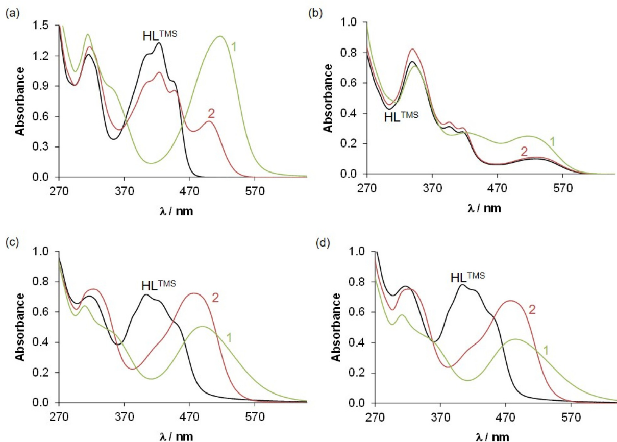
Fig. 2 UV-vis absorption spectra recorded for \text{HL}^{\text{TMS}} and its complexes (1, 2) after dissolution (a) in DMSO and at pH (b) 2.0, (c) 7.4 and (d) 11.7 ( c = 50 \mu\text{M} ; \ell = 1 \text{ cm} ; T = 25.0 \text{ }^\circ\text{C} ).
