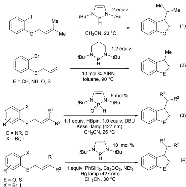
Scheme 12 Stoichiometric and catalytic ring closure reactions that implicate phosphorus-based radicals as an active species in the reaction.
