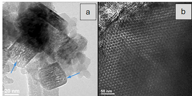
Fig. 14 Microscopic images of Pt/SBA-15_BEAl. 260 (a) TEM image of BEA with visible mesopores (some are indicated by blue arrows for easy identification), (b) TEM image of AlSBA-15 phase. Reproduced from ref. 260 with permission from Elsevier B.V., copyright 2019.
