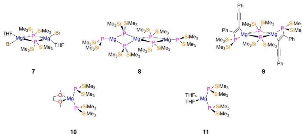
Fig. 3 \text{Mg } P'' complexes [\text{Mg}(\mu\text{-}P'')(\text{Br})(\text{THF})_2] ( 7 ), [\text{Mg}_3(\mu\text{-}P'')_4(P'')]_2 ( 8 ), [\text{Mg}(P''\text{C}(\text{Ph})\text{C}(\text{C}_2\text{Ph}))(\mu\text{-}P'')]_2 ( 9 ), [\text{Mg}(P'')_2(\text{DME})] ( 10 ), [\text{Mg}(P'')_2(\text{THF})_2] ( 11 ).
