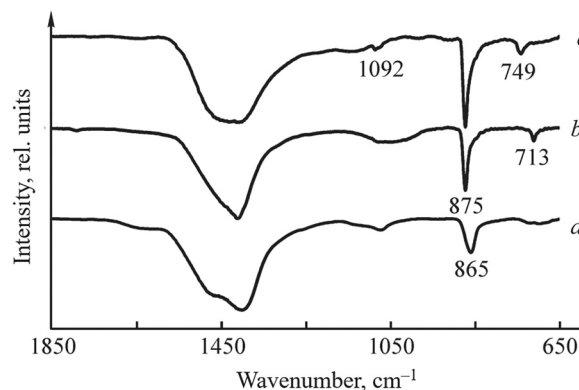
Fig. 5 IR spectra of (a) AOT-ACC, (b) calcite (heating ramp = 10\text{ }^\circ\text{C min}^{-1} ), and (c) vaterite (ramp = 1\text{ }^\circ\text{C min}^{-1} ). Adapted with permission from ref. 23 with permission from Royal Society of Chemistry, copyright 2013.
