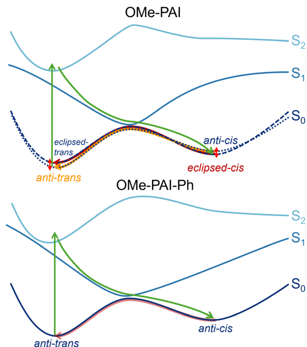
Fig. 6 Proposed mechanism of photoisomerization and thermal reversion for OMe-PAI and OMe-PAI-Ph. Photoinduced transformations are green and thermal processes are shades of red/orange. The different rotamer singlet surfaces for OMe-PAI are indicated with dotted and dashed lines with the lowest energy isomer shown in orange or red.
