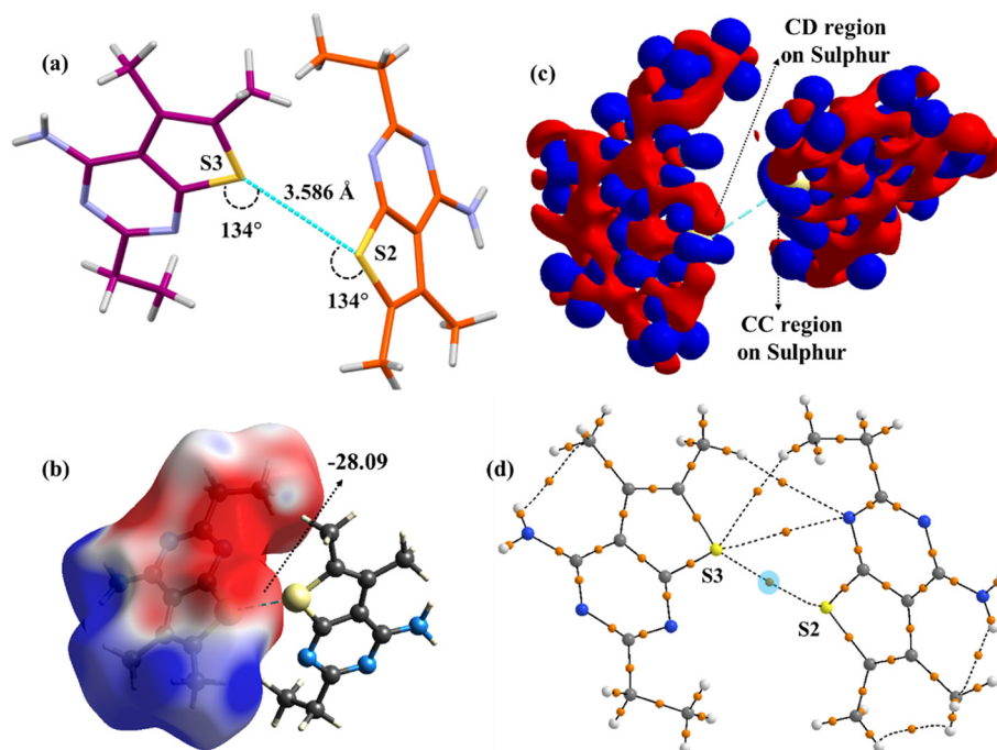
Fig. 17 (a) Distance and directionality of S\cdots S chalcogen interactions in compound 3 ; (b) MESP mapped over the Hirshfeld surface (values in \text{kJ mol}^{-1} ); (c) deformation density plot depicting the CC and CD regions; (d) QTAIM analysis validates the existence of bond critical points (highlighted in blue circles) in dimeric motifs.
