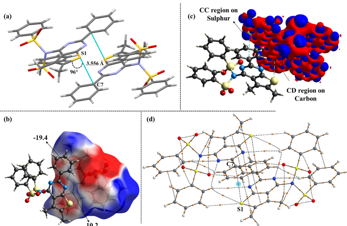
Fig. 16 (a) Distance and directionality of S\cdots C ( \pi -hole) tetrel interactions in compound 11 ; (b) MESP mapped over the Hirshfeld surface (values in \text{kJ mol}^{-1} ); (c) deformation density plot depicting the CC and CD regions; (d) QTAIM analysis validates the existence of bond critical points (highlighted in blue circles) in dimeric motifs.
