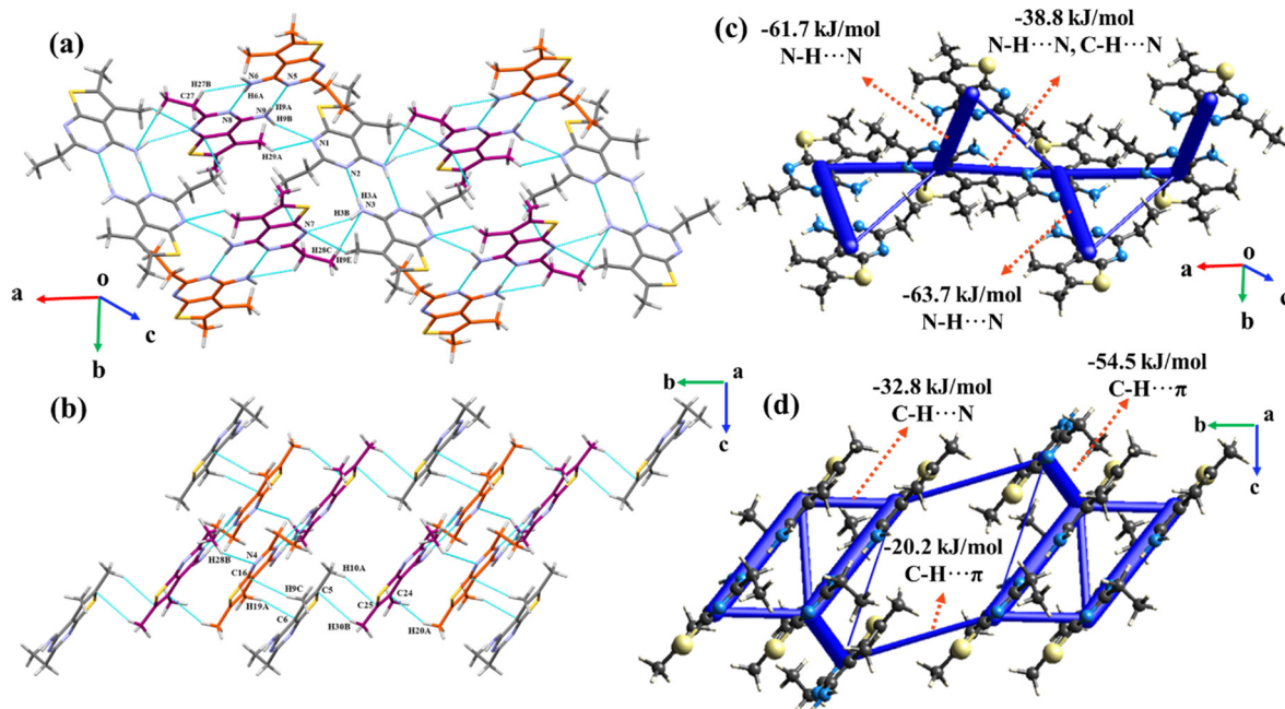
Fig. 4 (a) Herringbone arrangement formed via centrosymmetric N-H...N and C-H...N interactions in compound 3; (b) the overall packing of the molecule through C-H...π and C-H...N interactions; (c) and (d) energy frameworks depicting the total interaction energy from the N-H...N dimer along the ac -plane and C-H...π/N interactions in the bc -plane.
