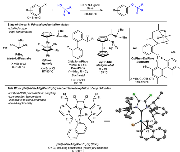
Scheme 1 Catalytic couplings of aryl halides with tertiary alcohols. In the depicted X-ray of the [\text{Pd}(\text{1-MeNAP})(\text{IPent}^{\text{Cl}})\text{Br}] catalyst, displacement ellipsoids are shown at the 50% probability level, and hydrogens are omitted for clarity (CCDC = 2492026). Selected bond lengths (Å): \text{C}_{\text{NHC}}\text{--Pd} = 2.049(3) , \text{Pd}\text{--C1} = 2.092(3) , \text{Pd}\text{--C2} = 2.242(3) , \text{Pd}\text{--C3} = 2.267(3) .
