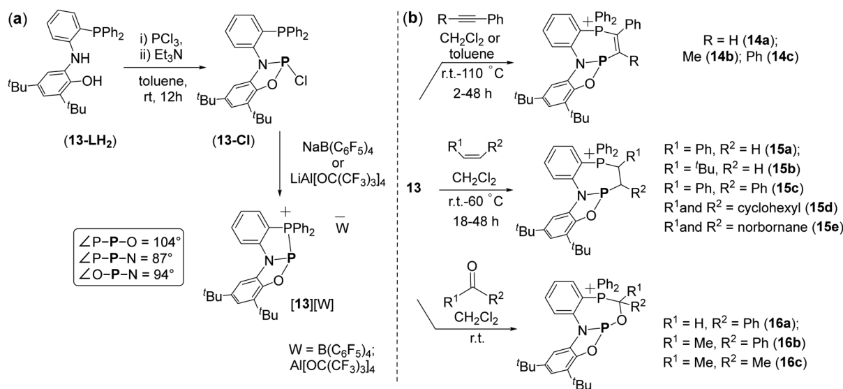
Fig. 8 (a) Synthetic scheme for the synthesis of [13][W] ; (b) phosphinophosphination of alkynes, olefins, and carbonyls with 13 .
