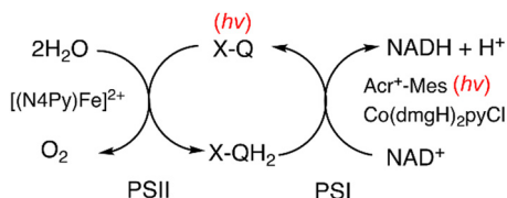
Scheme 17 Photocatalytic cycle for photocatalytic regiospecific NAD + reduction by H 2 O to produce 1,4-NADH and O 2 , achieved by combining PSI and PSII molecular models. Reprinted with permission from ref. 100. Copyright 2024, American Chemical Society.
