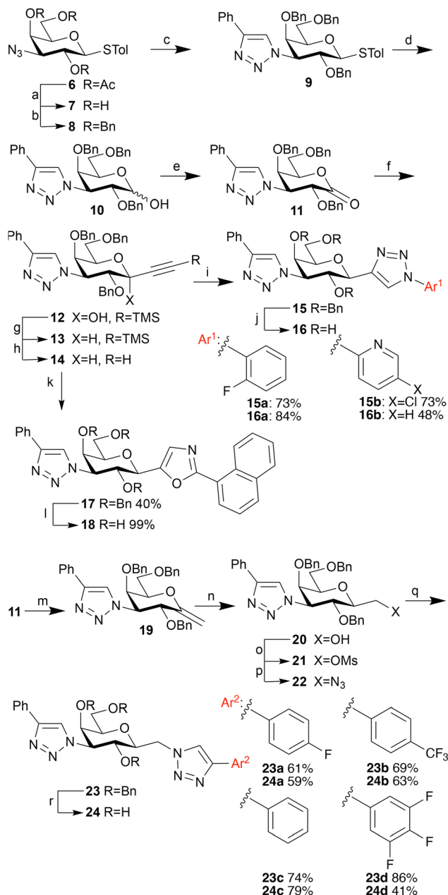
Scheme 2 Synthesis of 1,3-dideoxy-1-(aryltriazolyl)-3-(phenyltriazolyl)-β-D-galactopyranosides 15a–b , 1,3-dideoxy-1-(1-naphthylloxazolyl)-3-(phenyltriazolyl)-β-D-galactopyranoside 17 and 1-deoxy-3-(phenyltriazolyl)-1-(aryltriazolyl)-methyl-β-D-galactopyranosides 24a–d . (a) Sodium methoxide, methanol (dry), r.t., 2 h, 95%. (b) Sodium hydride, benzyl bromide, THF (dry), reflux 18 h, 84%. (c) Phenylacetylene, copper(i) iodide, triethylamine, ACN (dry), r.t., 18 h, 84%. (d) N -Bromosuccinimide, acetone/water, r.t., 10 min, 92%. (e) Dess–Martin periodinane, DCM (dry), r.t., 18 h, 99%. (f) Cerium(III) dichloride trimethylsilyl acetylde, THF (dry), –78 °C to r.t., 8 h, 78%. (g) Triethylsilane, boron trifluoride etherate, ACN/DCM (dry) 0 °C, 8 h, 60%. (h) Tetrabutylammonium fluoride, THF, r.t., 10 min, 91%. (i) Aryl azide, Copper(i) iodide, triethylamine, ACN (dry), r.t., 18 h. (j) Palladium hydroxide on carbon, cyclohexene/ethanol, reflux. (k) 1-Cyanonaphthalene, [Bis(trifluoromethanesulfonyl)imidate] (triphenylphosphine)gold(i), 8-methylquinoline N -oxide, 55 °C, sealed tube under nitrogen. (l) Palladium hydroxide on carbon, cyclohexene/ethanol, reflux. (m) Petasis reagent, toluene, 80 °C, 48 h, 63%. (n) Borane dimethyl sulfide, THF (dry), 0 °C, 12 h, then hydrogen peroxide, sodium hydroxide, THF/water, 0 °C, 2 h, 62%. Diastereoselectivity 4 : 1 β : α. (o) Mesyl chloride, pyridine, 0 °C, 2 h, 95%. (p) Sodium azide, DMF (dry), 95 °C, 2 h, 92%. (q) Aryl acetylene, copper(i) iodide, triethylamine, ACN (dry), r.t., 18 h. (r) Palladium hydroxide on carbon, cyclohexene/ethanol, 80 °C, 18 h.
