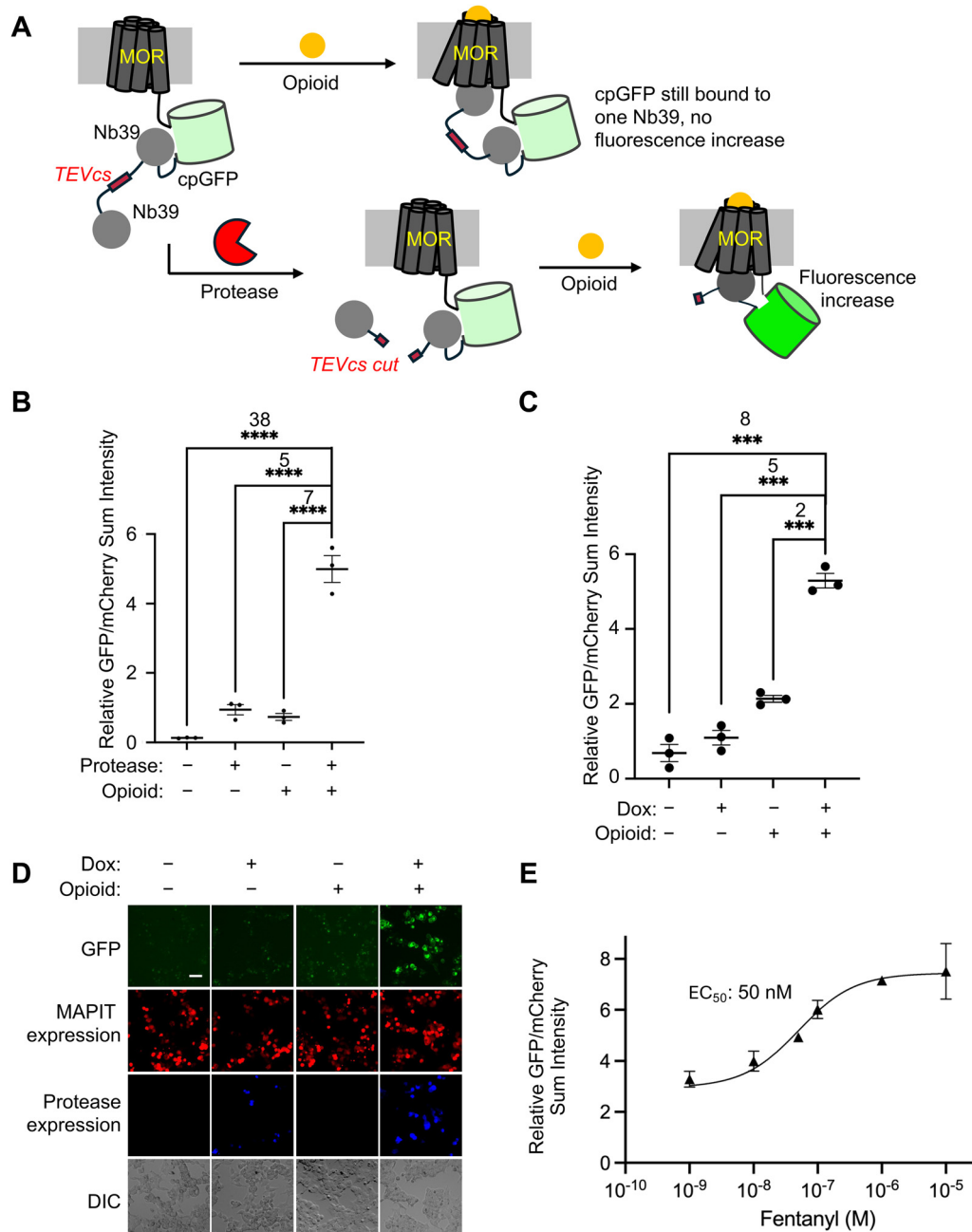
Fig. 4 MAPIT provides a protease-based time-gating for an opioid sensor in HEK cell culture. (A) Schematic of MAPIT. (B) Testing MAPIT with and without co-transfected TEVp and 10 μM loperamide. (C) Testing the doxycycline-induced expression of TEVp with the MAPIT sensor, with and without twenty-four hours of doxycycline and 10 μM loperamide. (D) Representative fluorescence images for (C). Scale bar: 50 μm. (E) Dose-response curve of Dox-MAPIT sensor for fentanyl. For fentanyl, the EC 50 range within 95% confidence is 19 to 123 nM. The mean is represented by each point in the plot ( n = 3 ). For (B) and (C) the thick horizontal bar is the mean value of three technical replicates ( n = 3 ). **** P < 0.0001 , *** P < 0.001 . The error bars represent SEM. The number above the stars is SBR between the two conditions and the stars indicate statistical significance. Significance was calculated using an unpaired, two-tailed student's t test.
