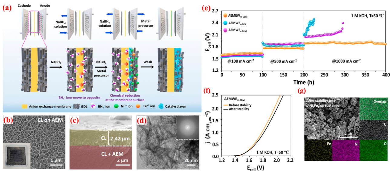
Fig. 8 (a) Schematic view of in situ ionomer-free m-CCM method; FE-SEM images of d- \text{Ni}_3\text{Fe}_1 CLs (b) arial view; (c) cross-section view; (d) HR-TEM image of d- \text{Ni}_3\text{Fe}_1 CL (inset: FFT pattern); (e) long-term durability study of AEMWEs at constant current densities; (f) polarization curves of AEMWEs using m-CCM with Sustainion X37-50 before and after long-term stability test; and (g) SEM an EDS mapping studies of d- \text{Ni}_3\text{Fe}_1 CLs on Sustainion X37-50 after the stability test. Reproduced with the permission from ref. 96. Copyright 2013, ACS.
