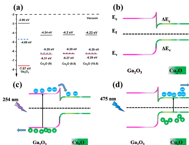
Fig. 6 Energy band structures of \text{Ga}_2\text{O}_3 and \text{Cu}_2\text{O} prepared at different pH values (a) before and (b) contact. The schematic diagram of carrier transport of \text{Cu}_2\text{O}/\text{Ga}_2\text{O}_3 heterojunction under (c) 254 (d) 475 nm illuminations.
