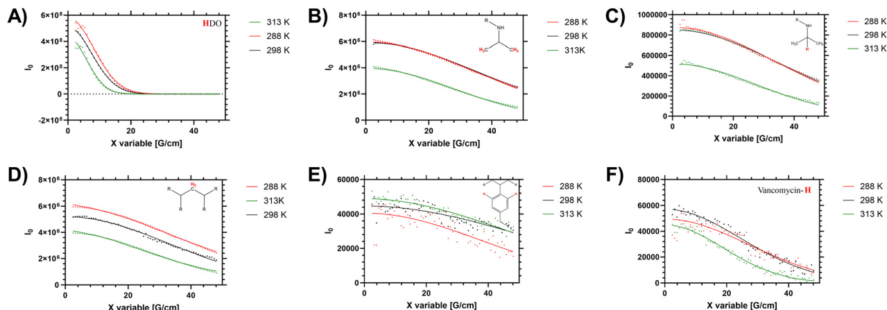
Fig. 2 Stejskal-Tanner plots of high resolution DOSY (48 gradient decay steps) of HB-PNIPAM-Vanc (polymer 2) showing varying diffusions of different components of branching architecture in D_2O at 288, 298 and 313 K. These represent peaks at (A) 4.69 ppm ( H_2O residue in solvent), (B) 1.1 ppm ( -CH_3 in PNIPAM isopropyl side chain), (C) 3.8 ppm ( -CH-(CH_3)_2 in PNIPAM isopropyl side chain), (D) 1.5 ppm ( CH_2 in polymer backbone), (E) 7.4 ppm (aromatic peaks from benzyl branching group), (F) 6.47 ppm (vancomycin aromatic-H peak from functional chain ends).
