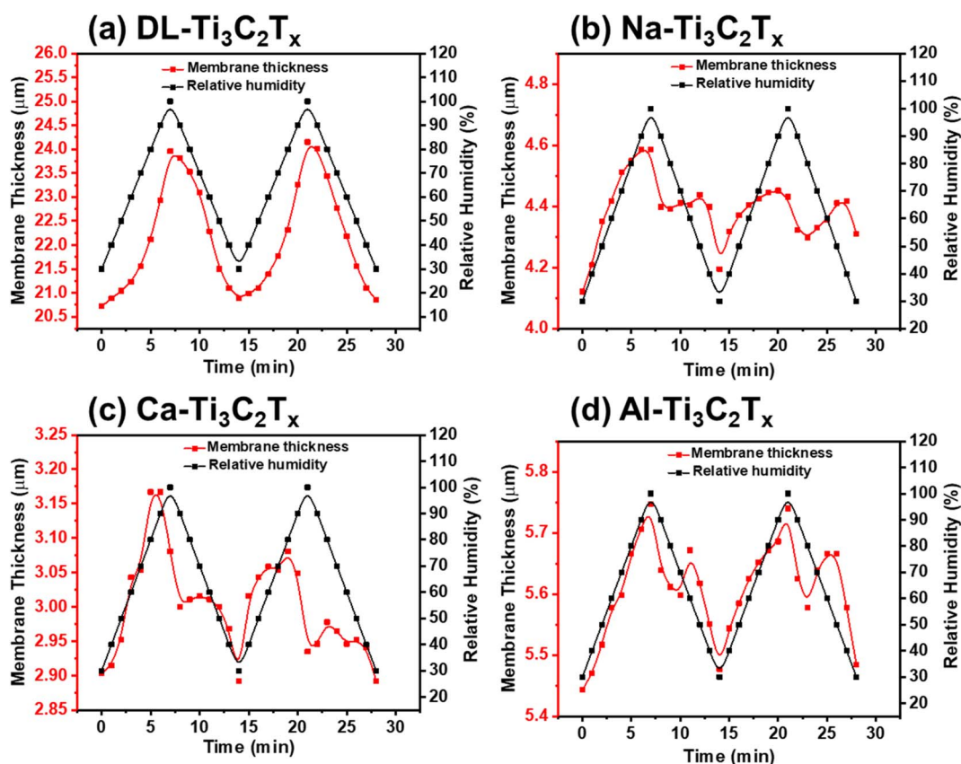
Fig. 4 Variation of membrane thickness in response to two cycles of relative humidity for (a) DL- \text{Ti}_3\text{C}_2\text{T}_x , (b) Na- \text{Ti}_3\text{C}_2\text{T}_x , and (c) Ca- \text{Ti}_3\text{C}_2\text{T}_x , and (d) Al- \text{Ti}_3\text{C}_2\text{T}_x . All measured thickness data points are within \pm 0.01 \mu\text{m} error.
