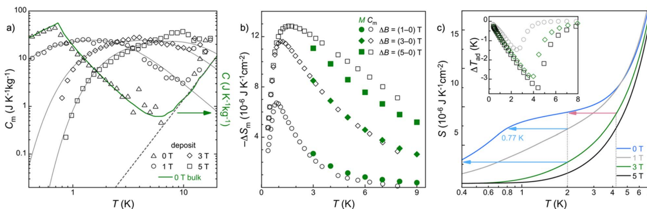
Fig. 2 (a) Temperature dependence of C_m for a film of Gd formate particles spin-coated with the Si substrate at 50 °C for different applied fields B . The zero-field C_p data for bulk Gd(HCOO) 3 is shown for comparison as a green line. Solid grey lines are calculated Schottky contributions for 1, 3 and 5 T. The dashed grey line is the lattice contribution calculated for a Debye temperature \theta_D = 168 K. 10a (b) Temperature dependence of -\Delta S_m per substrate area for different \Delta B , derived from magnetic heat capacity and magnetization data. (c) Temperature dependence of the total S per substrate area at different fields for the {Si + Gd(HCOO) 3 } spin-coated film. Arrows show the cooling produced by adiabatic demagnetization processes starting from either 2 or 4.2 K. Inset: temperature dependence of \Delta T_{ad} for adiabatic demagnetizations from 1, 3, and 5 T. The x axis represents the starting temperature of the adiabatic process.
